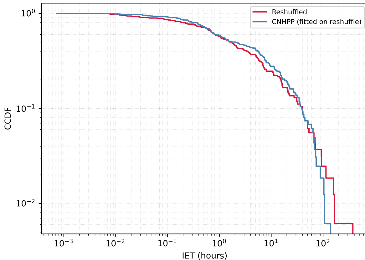
User 36162471 - Reshuffled vs CNHPP A_{\text{fit}}=0.3662
