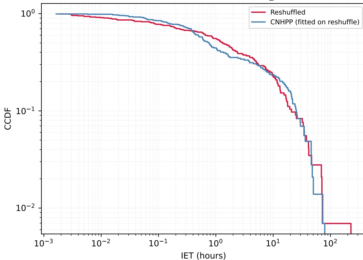
User 5213718005 - Reshuffled vs CNHPP A_{\text{fit}}=0.6306
