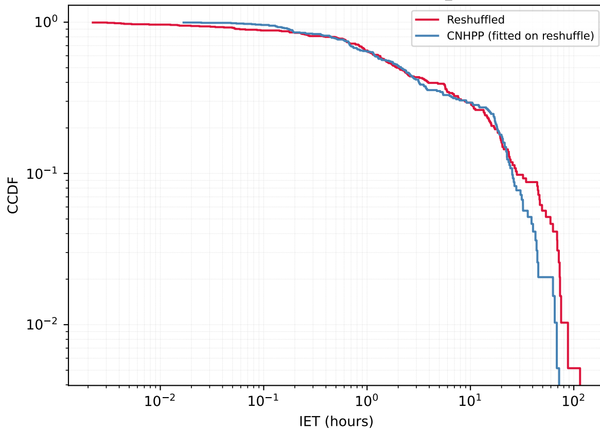
User 6111348138 - Reshuffled vs CNHPP A_{\text{fit}}=0.3361
