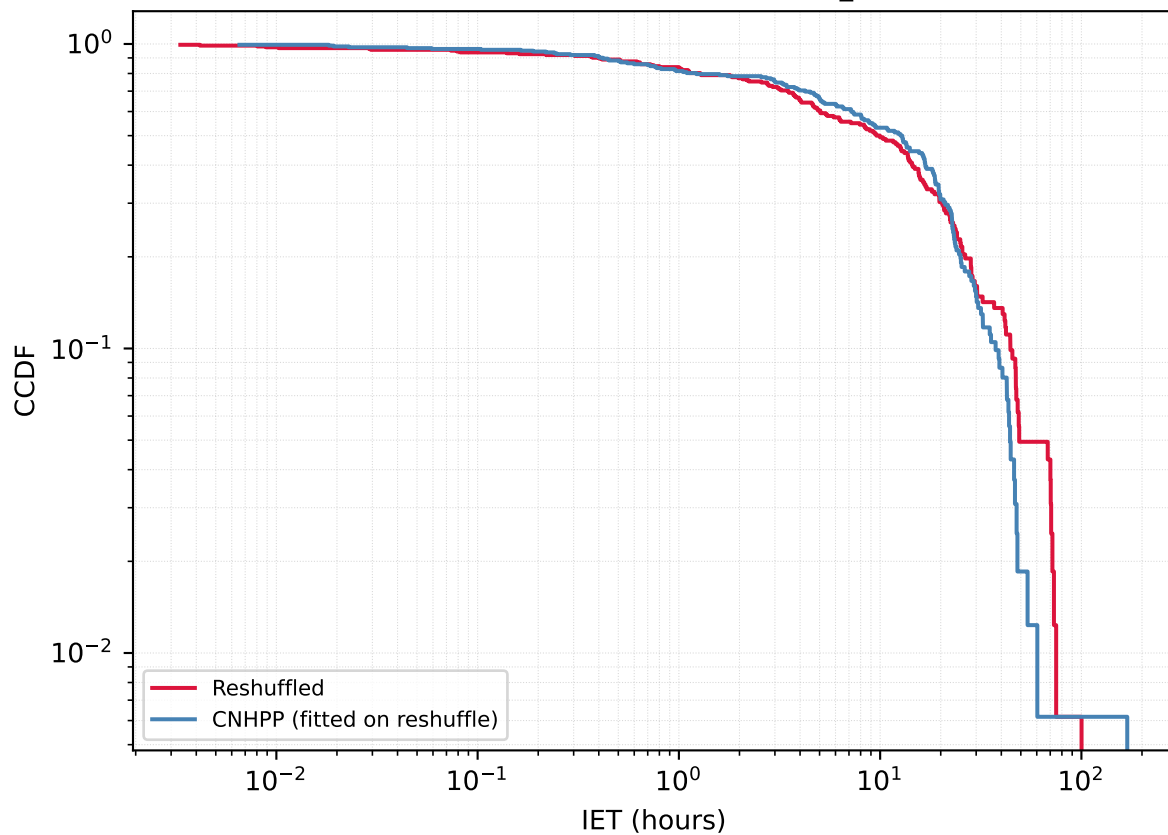
User 4473225 - Reshuffled vs CNHPP A_{\text{fit}}=0.2221
