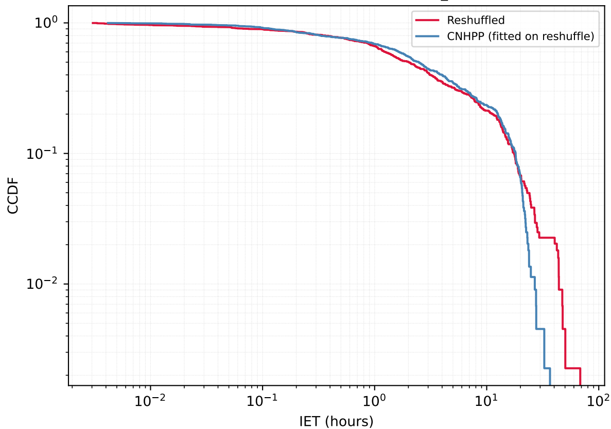
User 323309626 - Reshuffled vs CNHPP A_{\text{fit}}=0.3924
