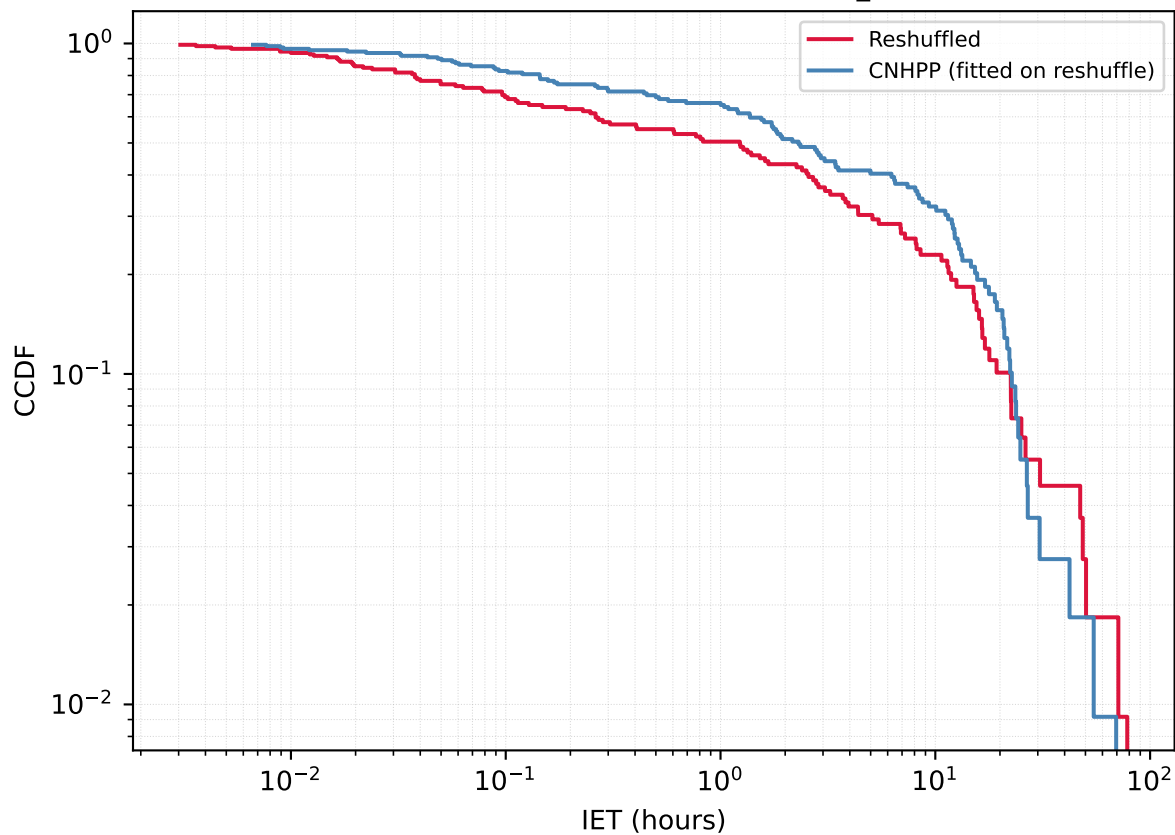
User 675391573 - Reshuffled vs CNHPP A_{\text{fit}}=0.9763
