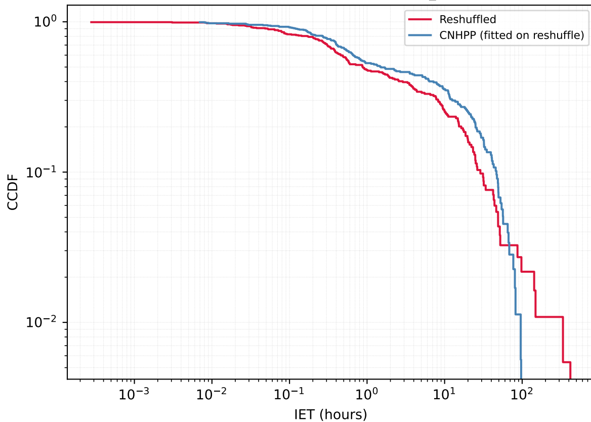
User 17798588 - Reshuffled vs CNHPP A_{\text{fit}}=0.4129
