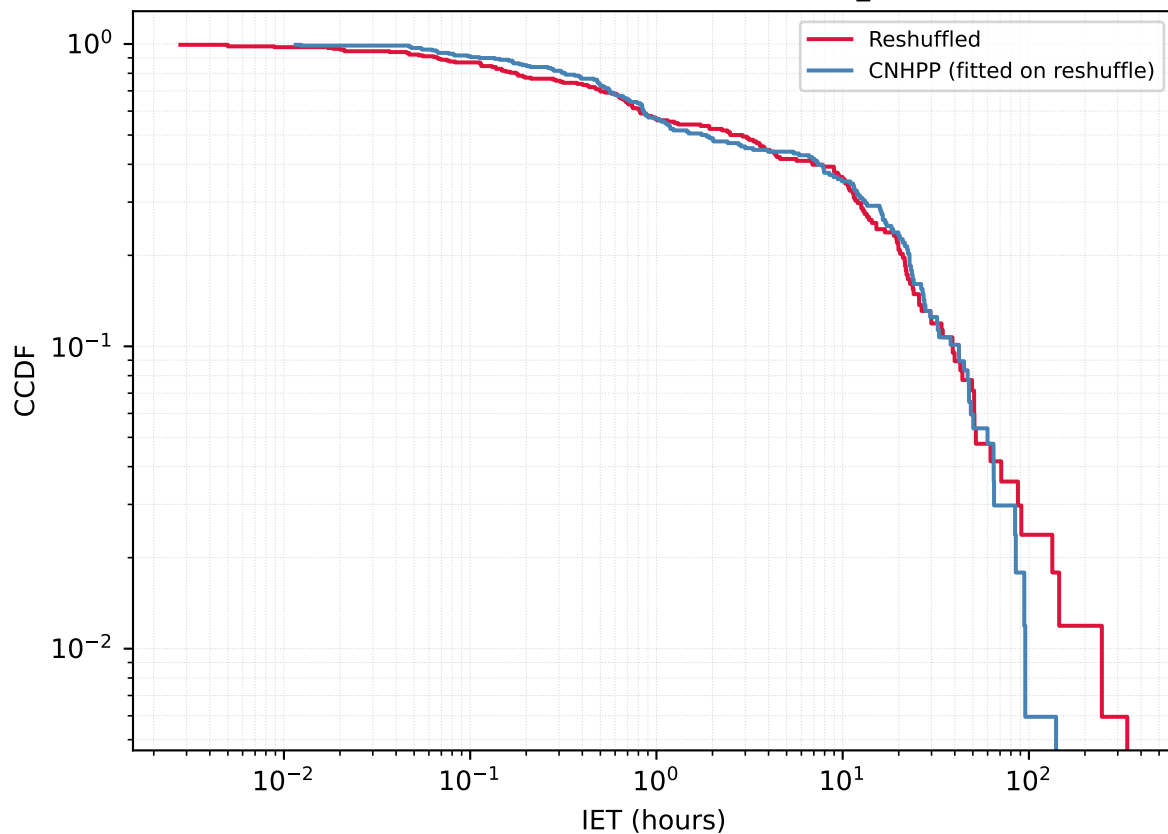
User 185880661 - Reshuffled vs CNHPP A_{\text{fit}}=0.4519
