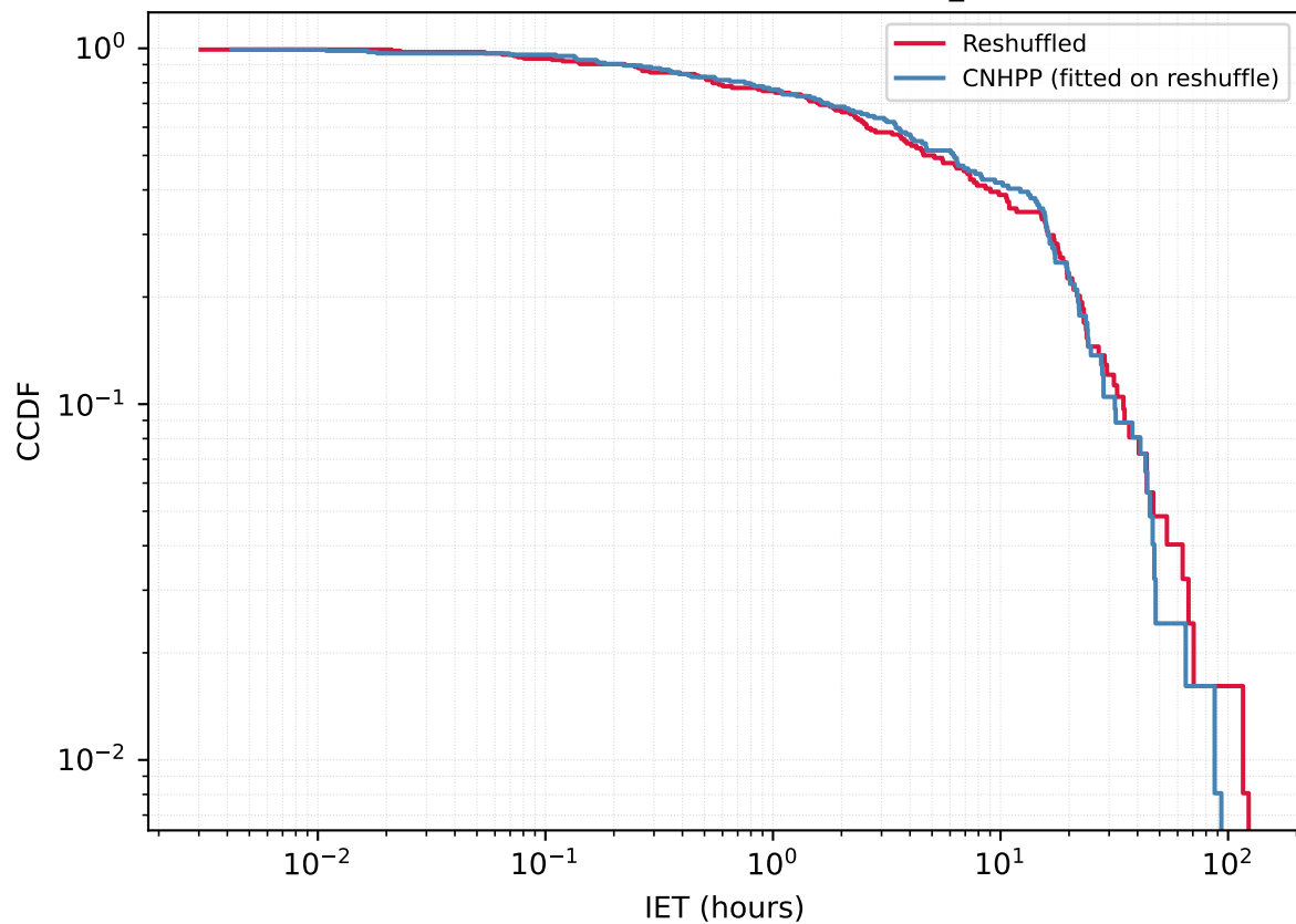
User 458678536 - Reshuffled vs CNHPP A_{\text{fit}}=0.4362
