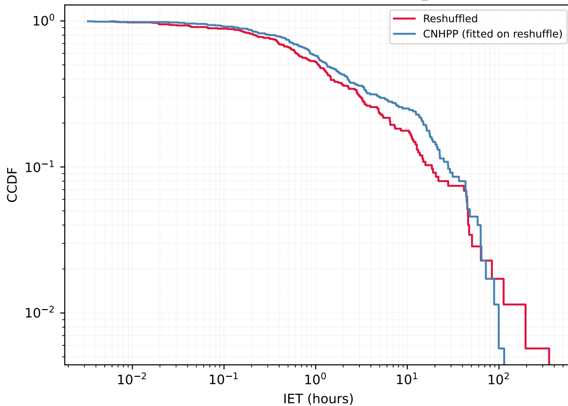
User 6947363606 - Reshuffled vs CNHPP A_{\text{fit}}=0.2395
