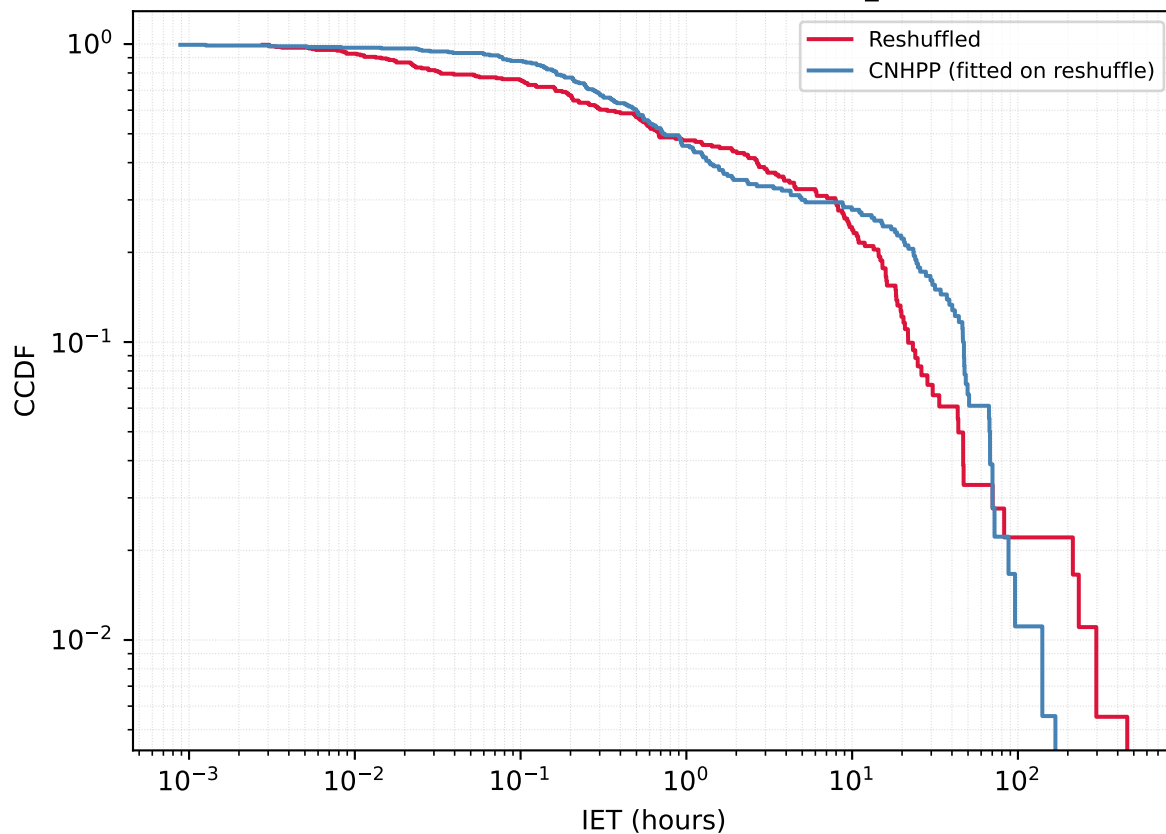
User 5719413972 - Reshuffled vs CNHPP A_{\text{fit}}=0.7818
