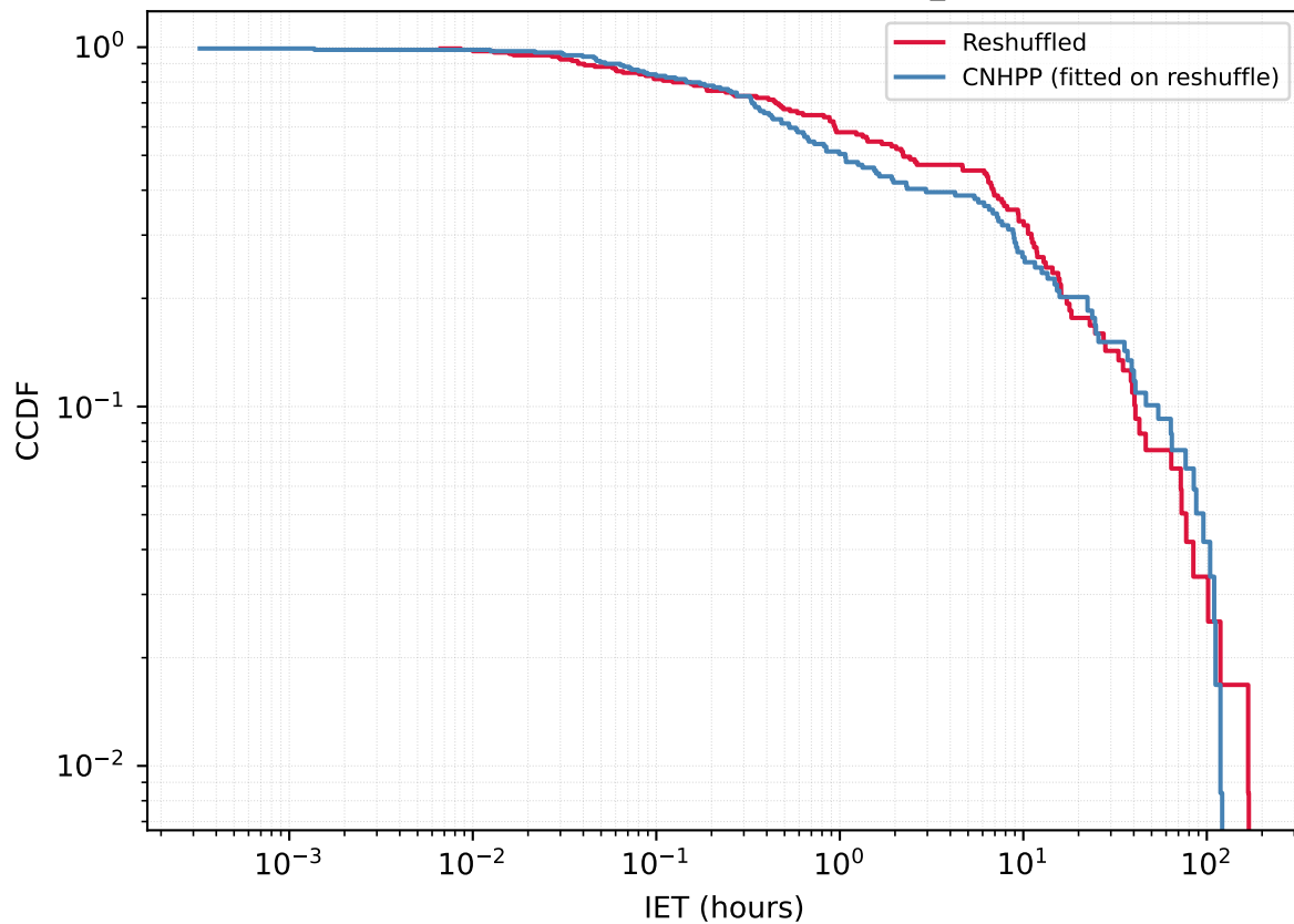
User 5357949 - Reshuffled vs CNHPP A_{\text{fit}}=0.7787
