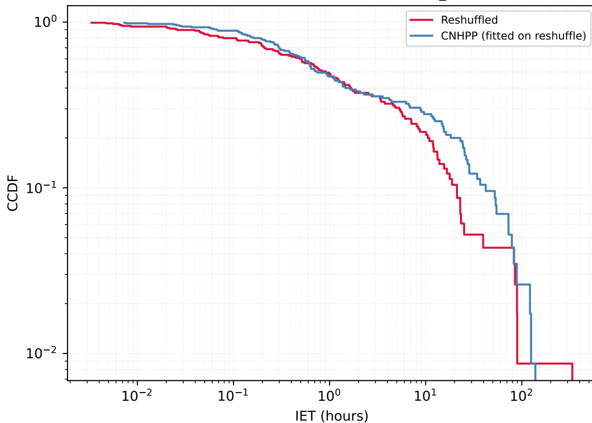
User 1083421726 - Reshuffled vs CNHPP A_{\text{fit}}=0.3539
