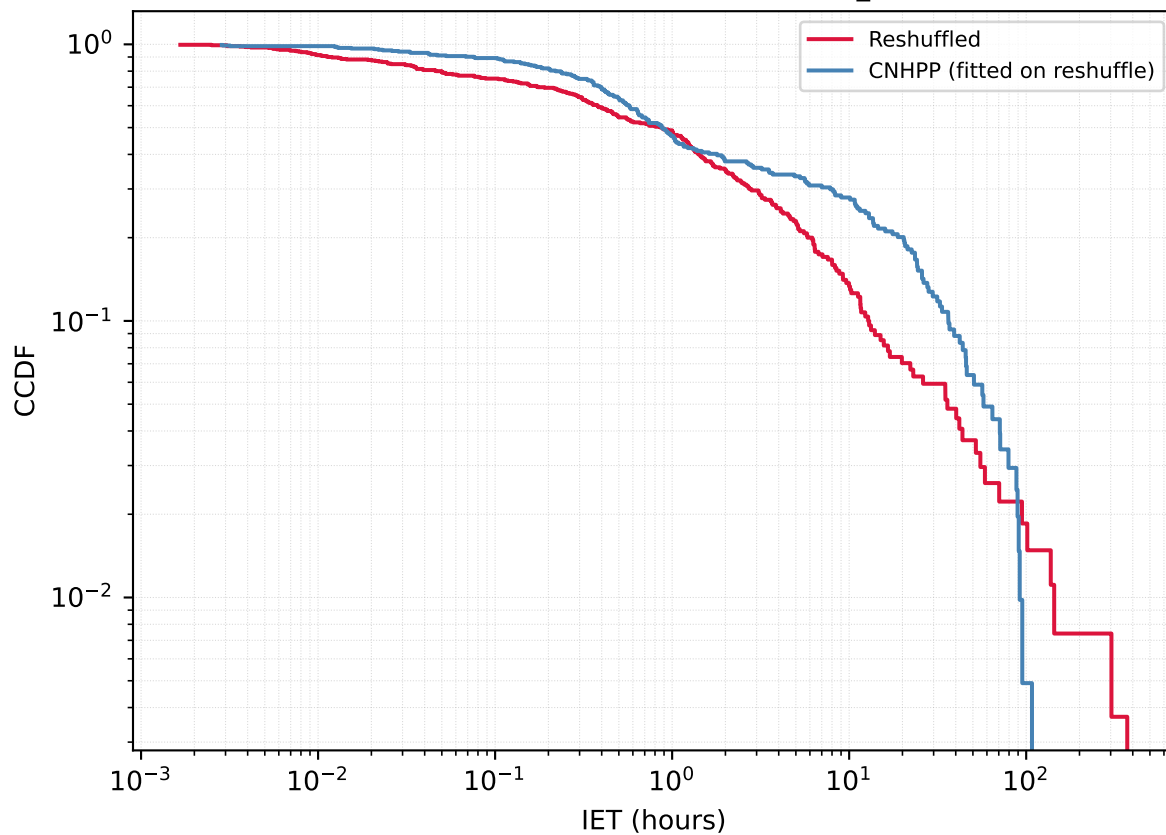
User 145800528 - Reshuffled vs CNHPP A_{\text{fit}}=0.6773
